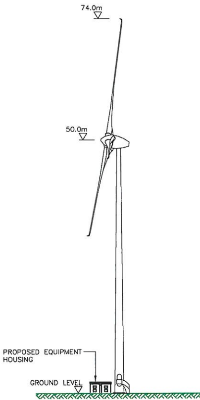
SIDE ELEVATION (1:500)
