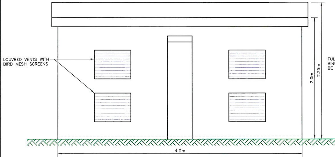
SIDE VIEW (1:25)
