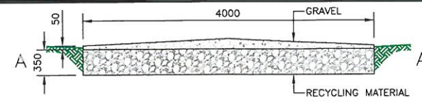
ACCESS ROAD CONSTRUCTION DETAIL SECTION A-A (1:50)
