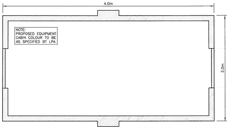
PLAN VIEW (1:25)
