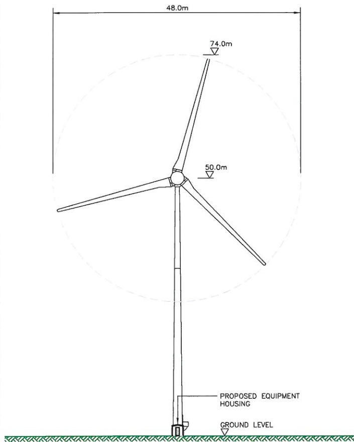
FRONT ELEVATION (1:500)
