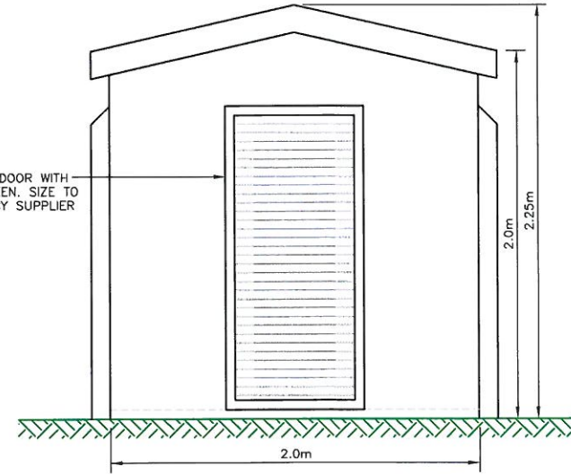
FRONT/REAR VIEW (1:25)
